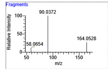
Xylazine 甲苯噻嗪
